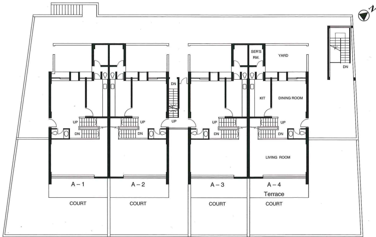
GROUND FLOOR (BLOCK A)
