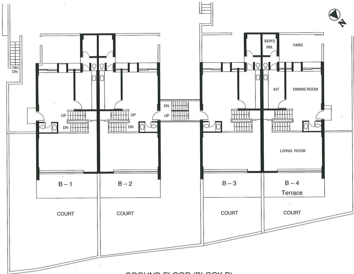
GROUND FLOOR (BLOCK B)
